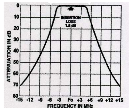
5044-8-2 Response Curve (Typical) 5 MHz Bandwidth (806-960 MHz)
