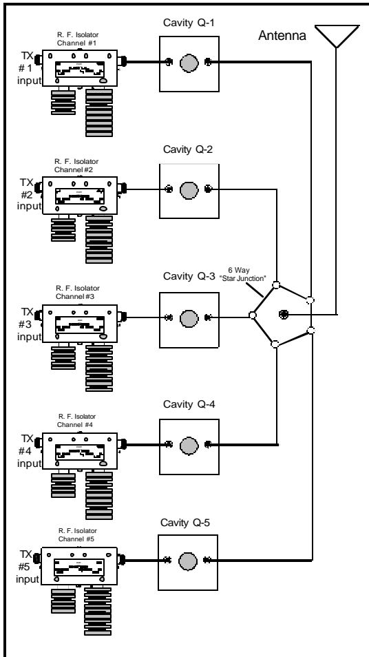
Figure 7 Star Junction Combiner
