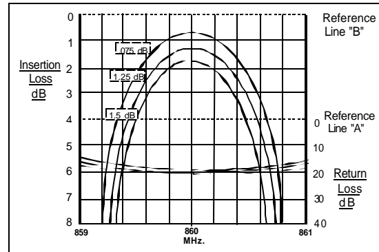
Figure 5 Band pass cavity responses at different coupling factors
