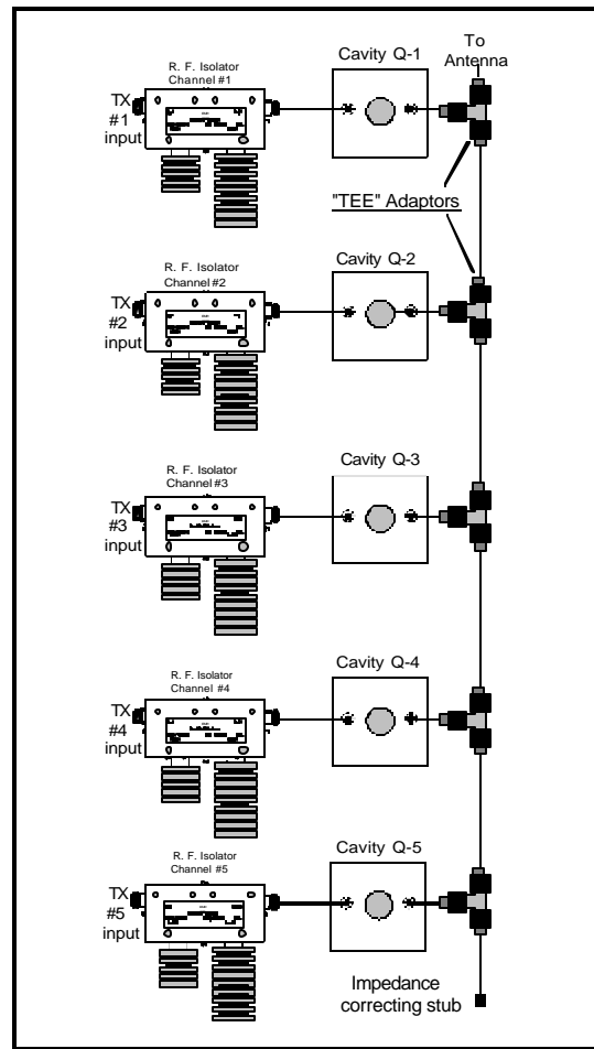
Figure 8 Line Segment Combiner
