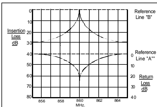
Figure 2 Response of single 7" square cavity Set for 1.2 dB insertion loss, shown on 10 dB per division vertical resolution.
