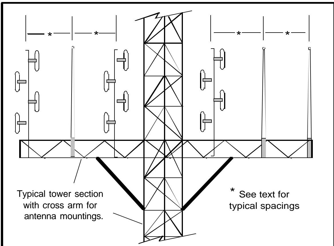
Figure 10 Horizontally Mounted Transmitting Antennas
